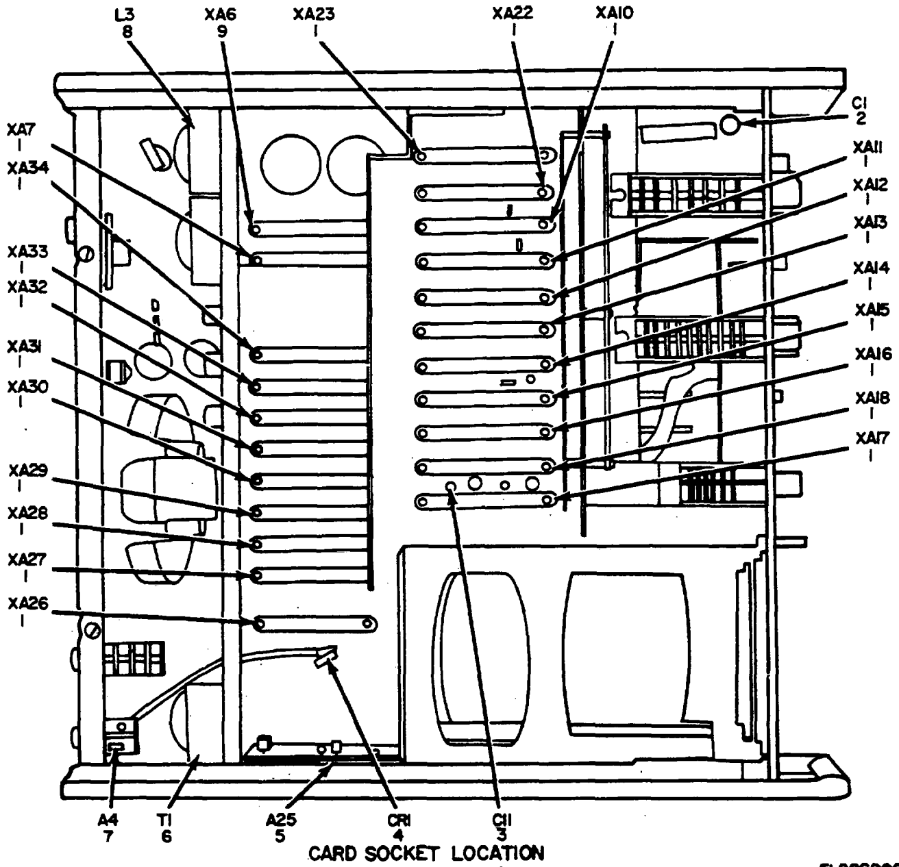
Figure 6. Electronic Counter CP-772A/U, Bottom View (Sheet 1 of 2).
