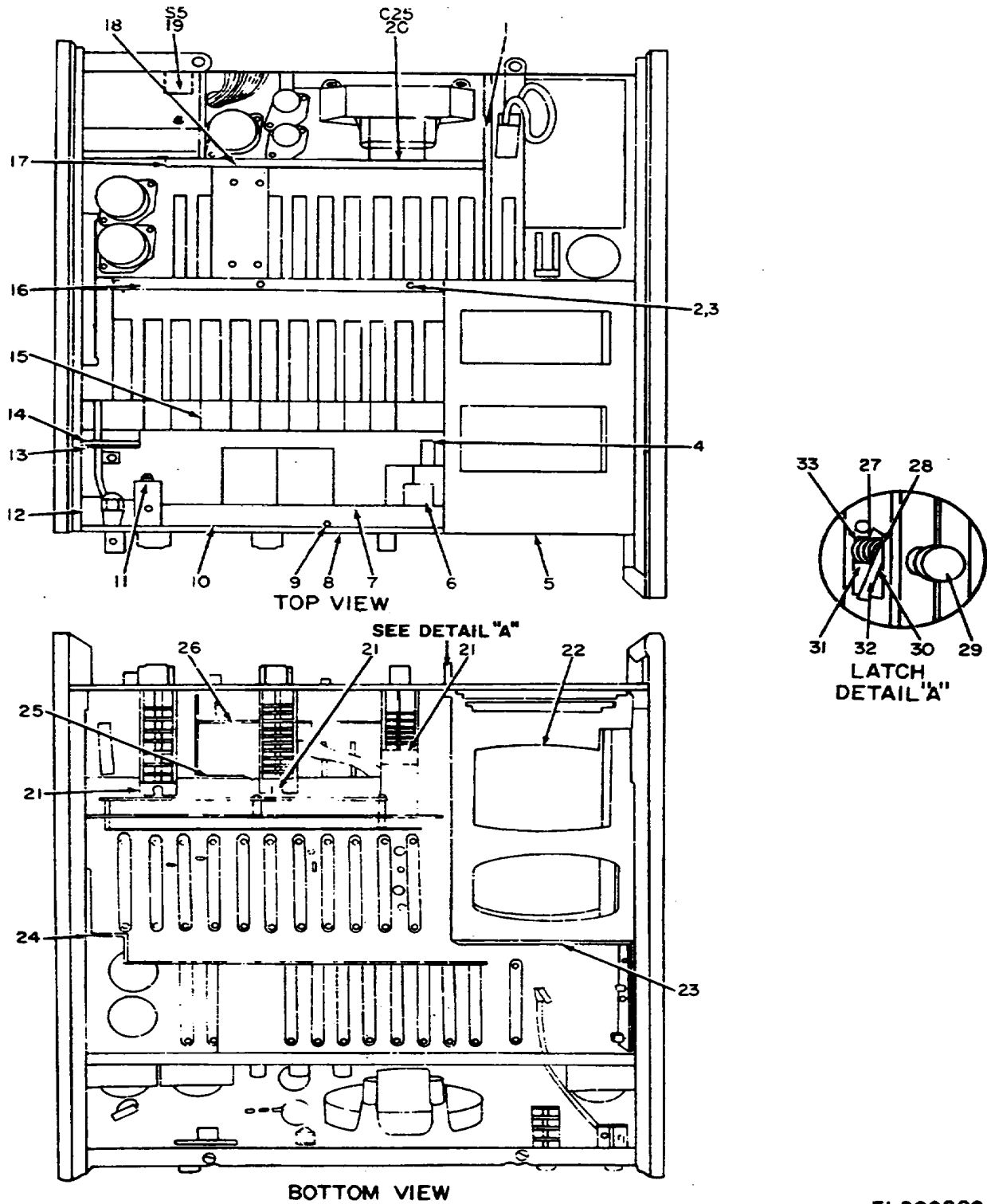
Figure 7. Electronic Counter CP-772A/U, Top and Bottom Views.
