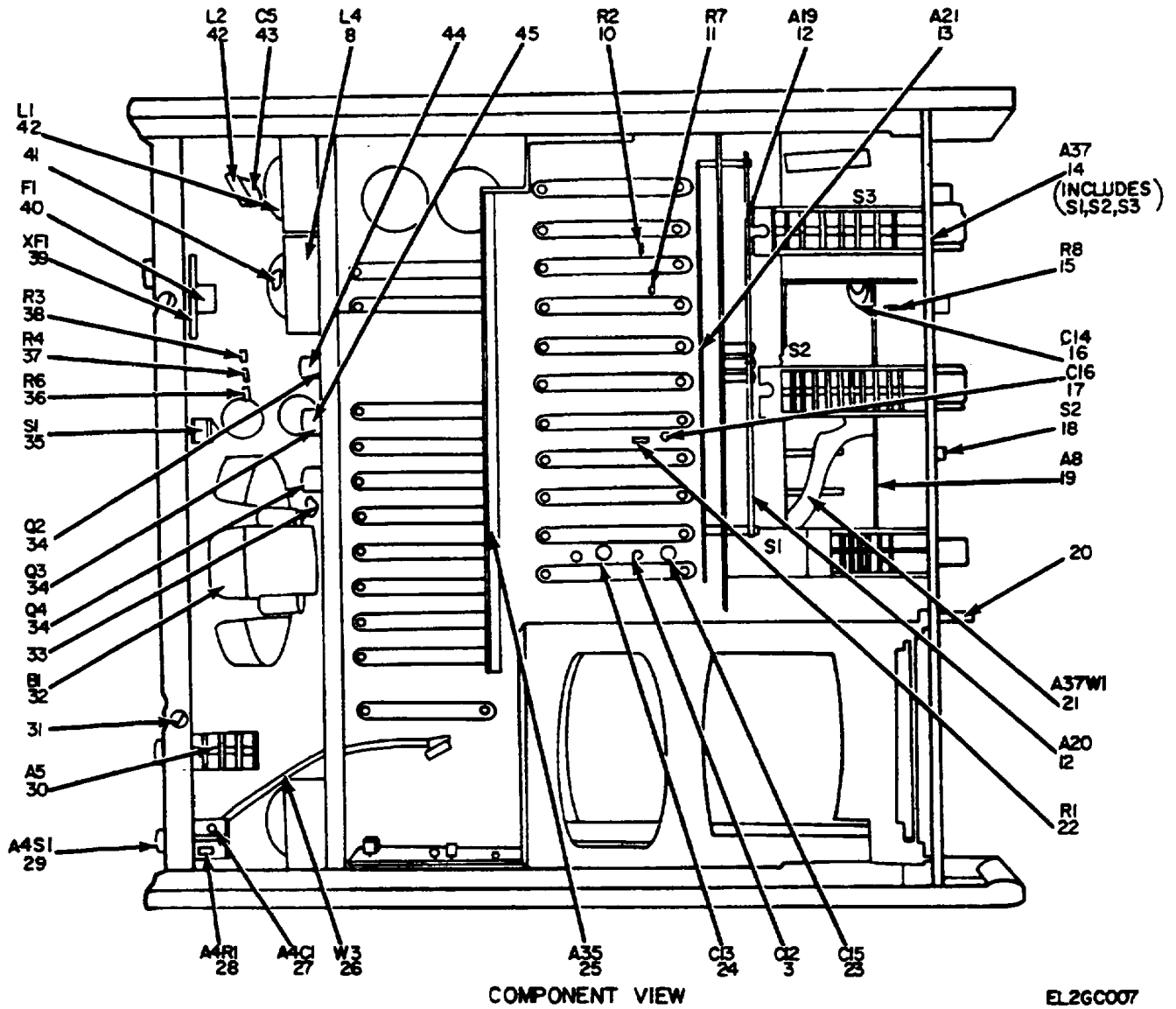
Figure 6. Electronic Counter CP-772A, Bottom View (Sheet 2 of 2).
