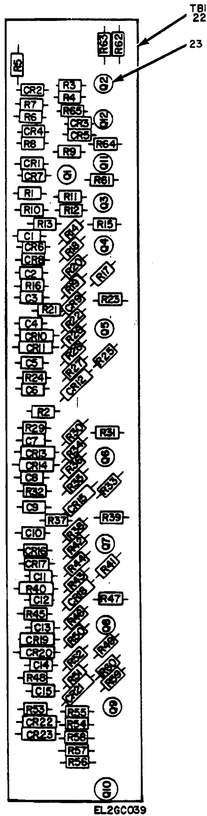
Figure 26. Electronic Counter CP-772A/U, Printed Circuit Board A35 (Sheet 1 of 2).
