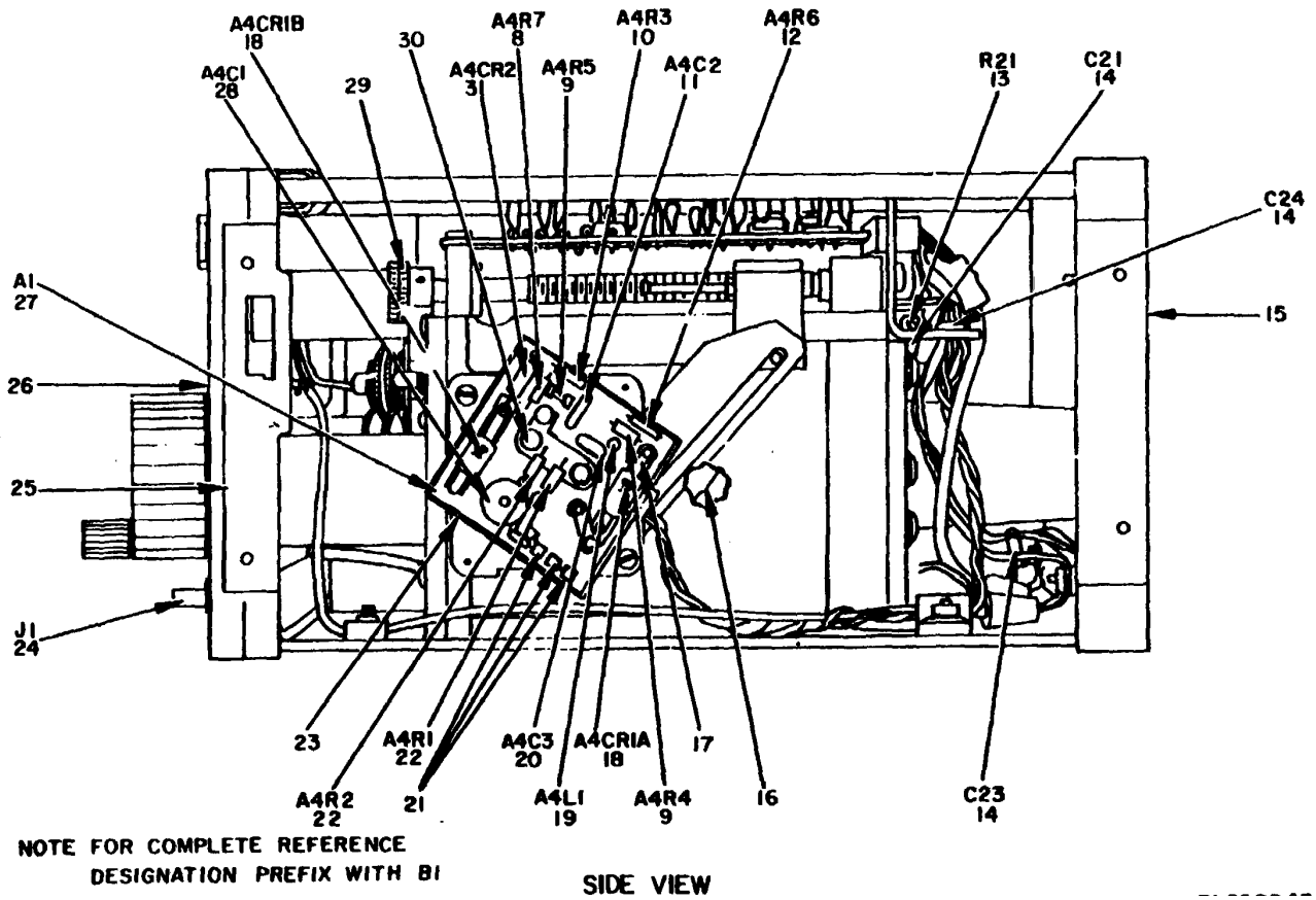
Figure 28. Frequency Converter CV-2002/U (Sheet 2 of 2).
