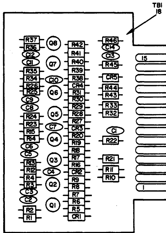
Figure 25. Electronic Counter CP-772A/U, Printed Circuit Boards A29 thru A34 (Sheet 1 of 2).
