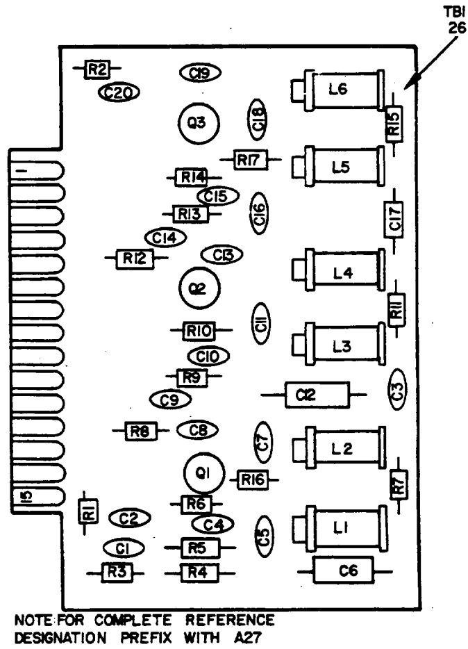
Figure 23 . Electronic Counter CP-772A/U, Printed Circuit Board A27 (Sheet 1 of 2).
