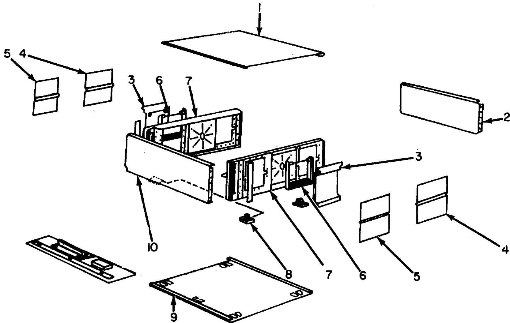
Figure 3. Electronic Counter CP-772A/U, Exploded View
