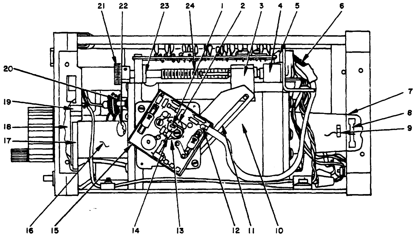
Figure 31. Frequency Converter CV-2002/U, Components.
