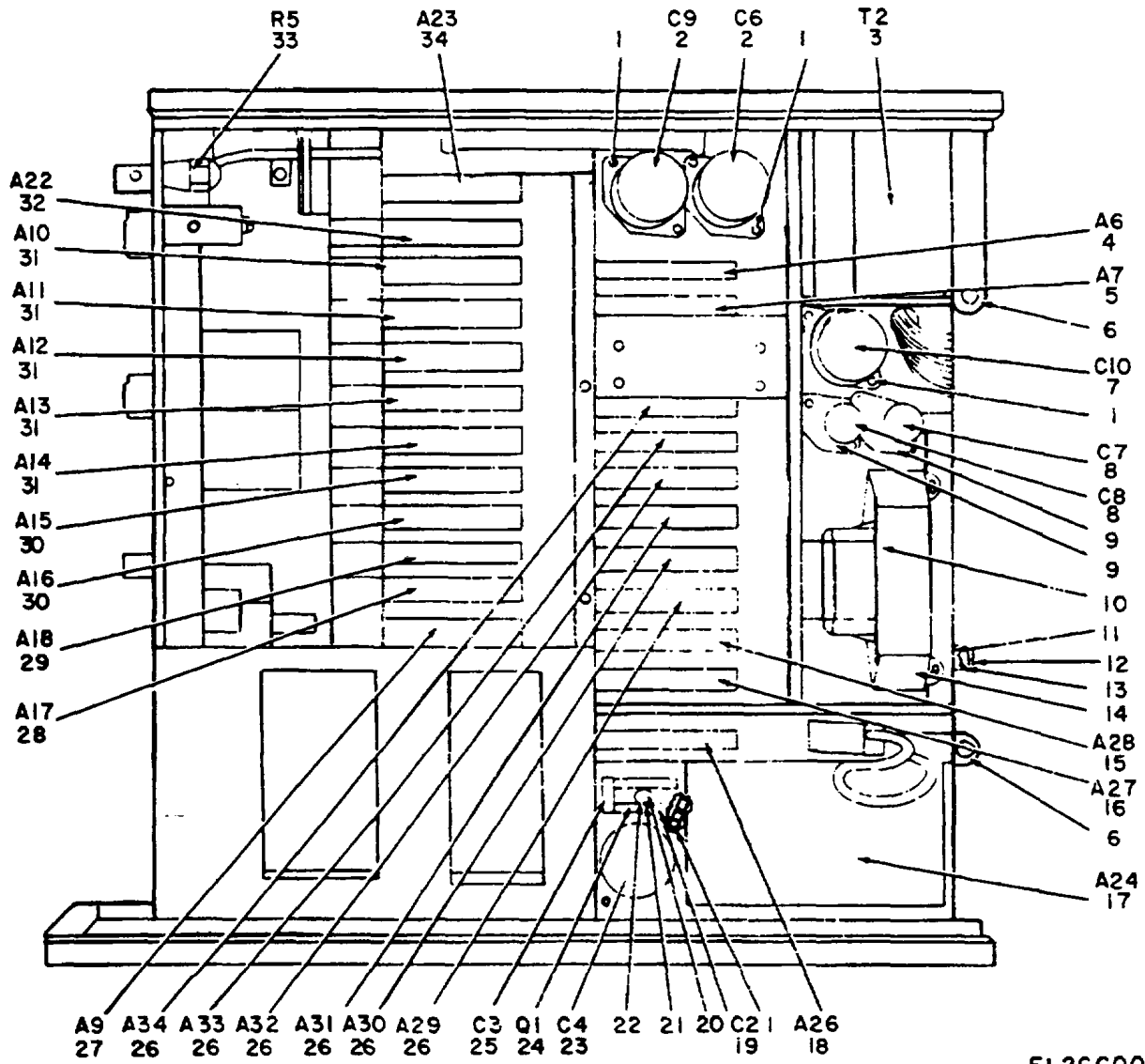
Figure 5. Electronic Counter CP-77A/U, Top View.
