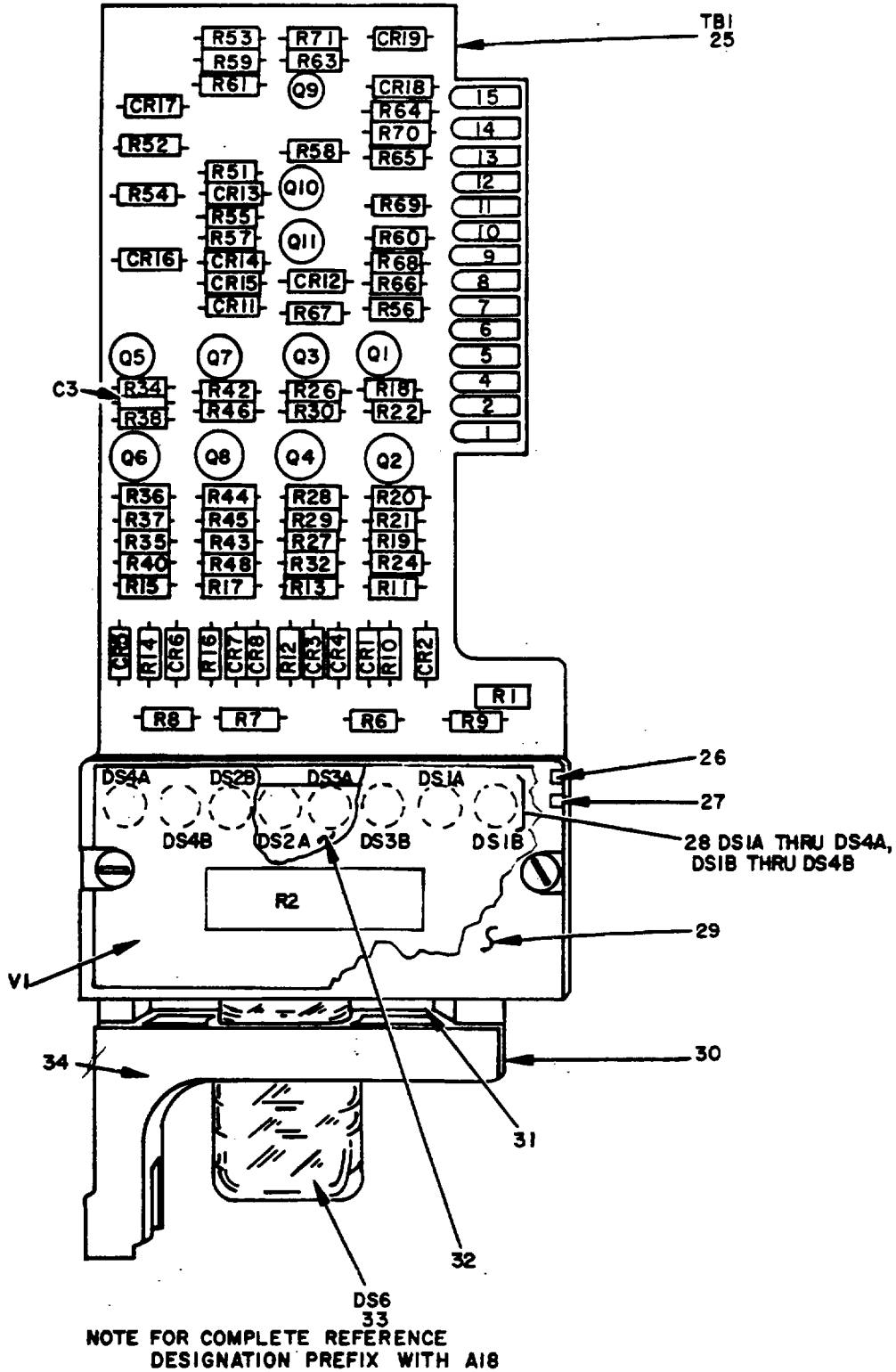
Figure 16. Electronic Counter CP-772A/U, Printed Circuit Board A18 (Sheet 1 of 2).
