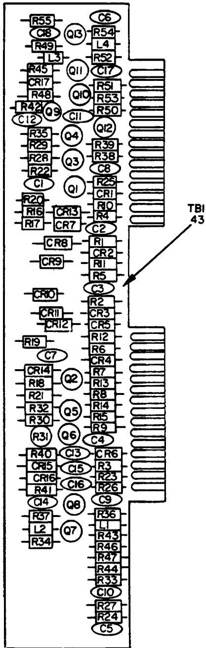
Figure 18 . Electronic Counter CP-772A/U, Printed Circuit Board A21 (Sheet 1 of 2).
